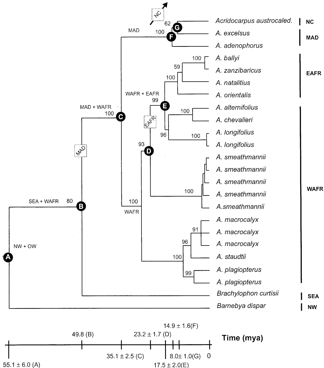
FIG. 2. Maximum-likelihood tree topology ( -\ln L = 7945.63 ) estimated from combined ITS, ndhF , and trnL-F data showing rate-smoothed branch lengths. Bootstrap support values \geq 50\% are shown on branches. The nodes labeled A–G correspond to ancestral areas estimated from dispersal-vicariance analysis reconstructions, which are shown next to the relevant nodes. The age estimate for the basal New World–Old World disjunction at node A was previously estimated by Davis et al. (2002a). Divergence times were calculated on this tree by calibrating the ancestral node (B) of the acridocarpoids at 49.8 million years ago. This age estimate was derived from the global analysis of Malpighiaceae from PHYC and ndhF data in this study. Age estimates for disjunctions labeled A–G are indicated on the scale bar below. Boxed areas indicate inferred dispersal events from ancestral area (indicated at stem node) into the area specified along the branch in the box. Modern distributions of species are indicated to the right. EA, East Africa (includes Arabia, and southern coastal Africa); MAD, Madagascar; NC, New Caledonia; NW, New World; OW, Old World; SEA, Southeast Asia; WA, West Africa (includes western and central Africa).
